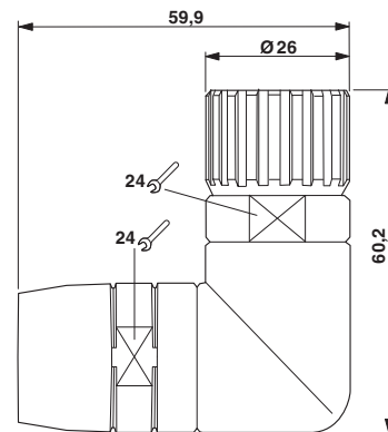
Dimensioned drawing
