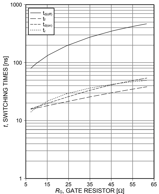
Figure 8. Typical switching times as a function of gate resistor (inductive load, T vj =150°C, V CE =400V, V GE =0/15V, I C =30A, Dynamic test circuit in Figure E)
