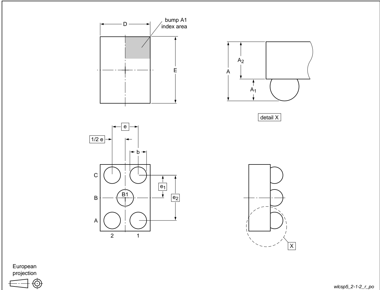
Fig 1. Package outline IP4059CX5/LF (WLCSP5)
