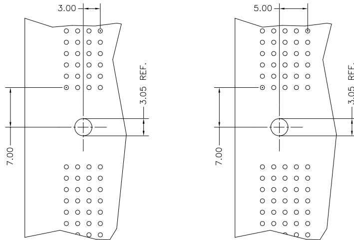
RECOMMENDED HOLE PATTERN WHEN STACKED BESIDE A STANDARD 4 MOD METRAL HEADER COMPONENT SIDE
