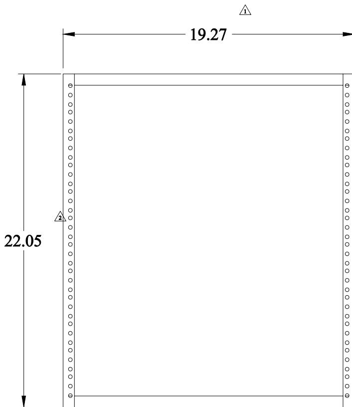
FRONT VIEW
