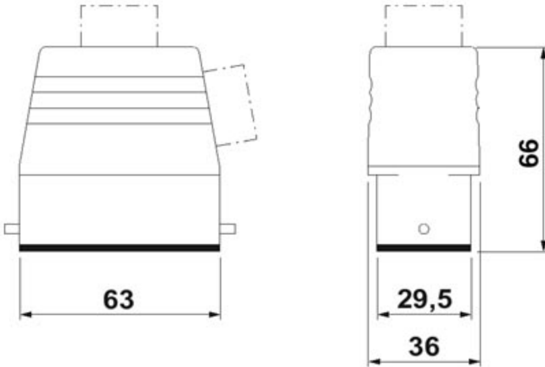
Dimensioned drawing
