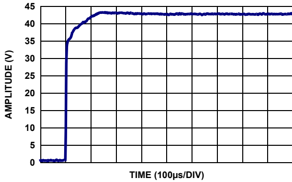
FIGURE 56. DFET RISE
