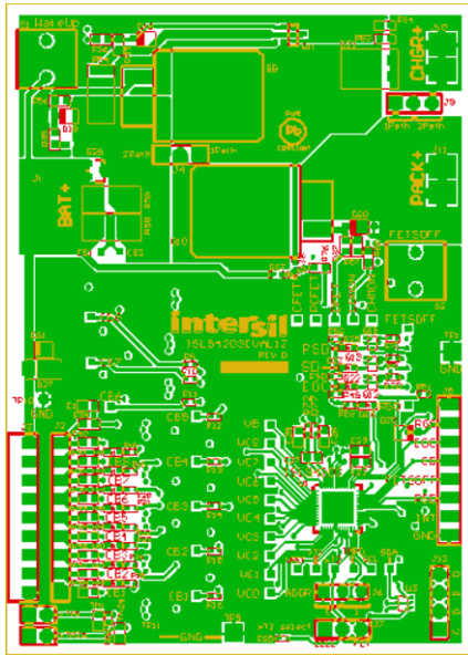
FIGURE 50. TOP LAYER
