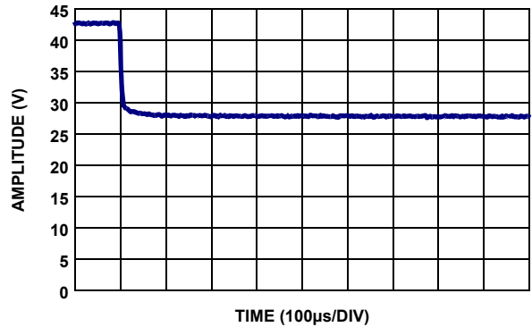
FIGURE 59. CFET FALL
