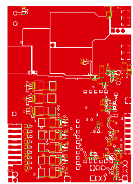
FIGURE 53. BOTTOM LAYER
