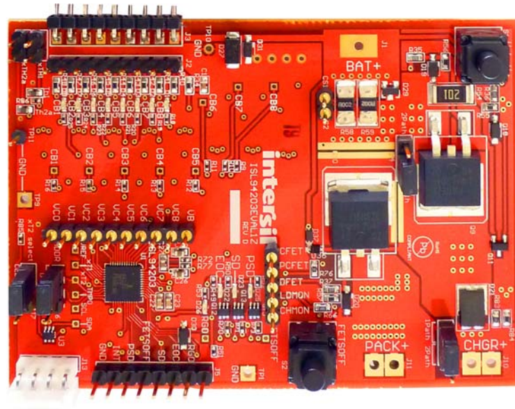
FIGURE 1. ISL94203EVKIT1Z EVALUATION BOARD
