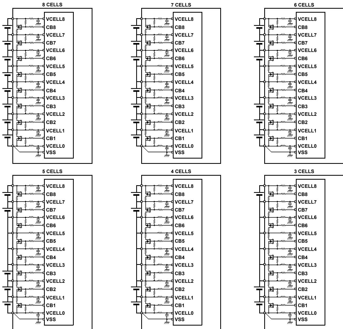
FIGURE 55. BATTERY CONNECTION OPTIONS USING THE ISL94203EVKIT1Z BOARD
