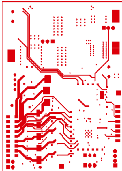
FIGURE 52. MIDDLE LAYER 2
