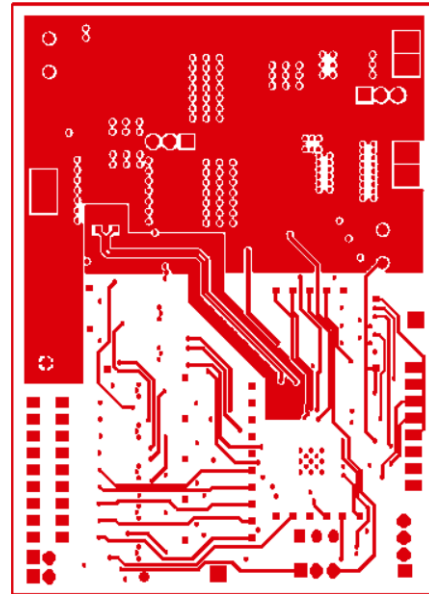
FIGURE 51. MIDDLE LAYER 1
