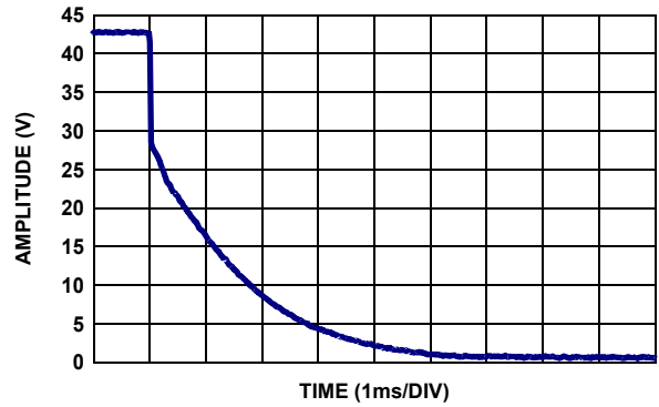
FIGURE 57. DFET FALL
