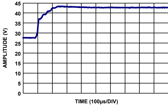
FIGURE 58. CFET RISE
