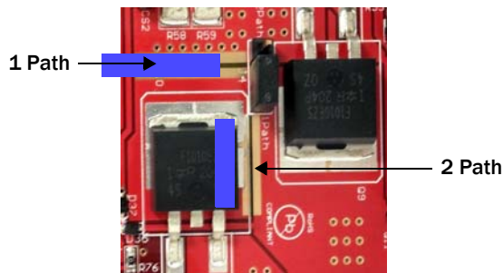
FIGURE 54. SOLDER JUMPERS FOR HIGHER CURRENT
