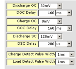
FIGURE 32. CURRENT LIMITS
