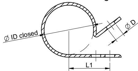
sectional drawing A-A
