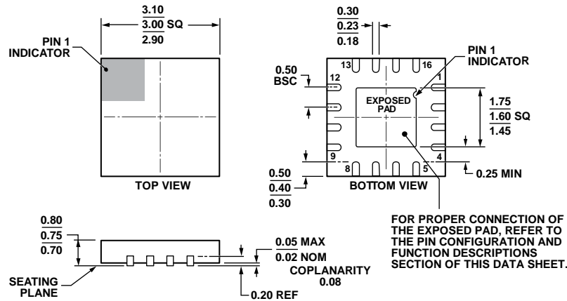
Figure 49. 16-Lead Lead Frame Chip Scale Package [LFCSP] 3 mm x 3 mm Body and 0.75 mm Package Height (CP-16-22) Dimensions shown in millimeters
