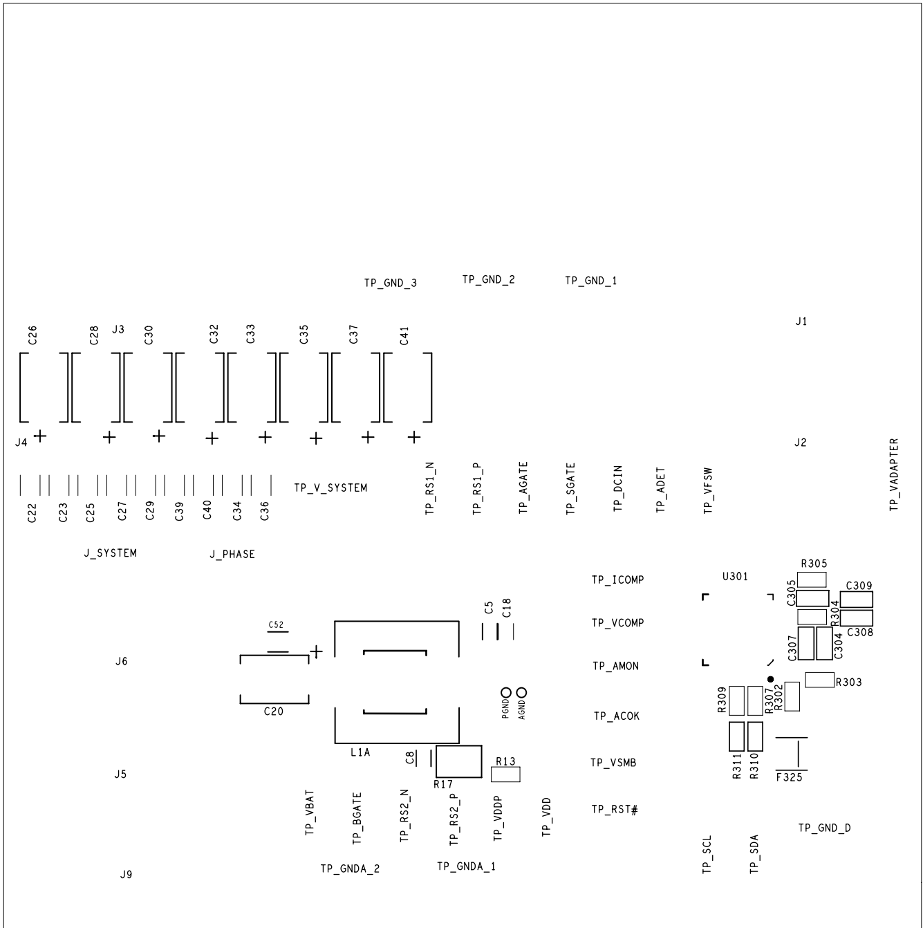
FIGURE 18. BOTTOM SILKSCREEN
