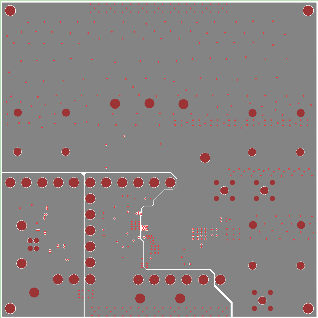
FIGURE 20. LAYER 2 COPPER
