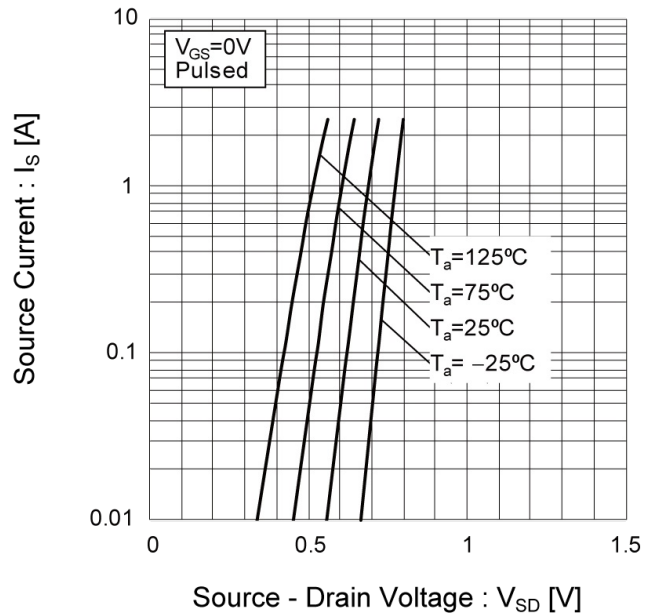
Fig.19 Source Current vs. Source Drain Voltage
