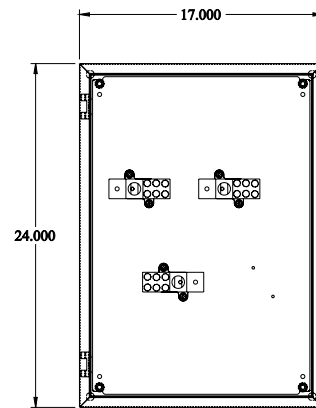
FRONT VIEW - COVER REMOVED
