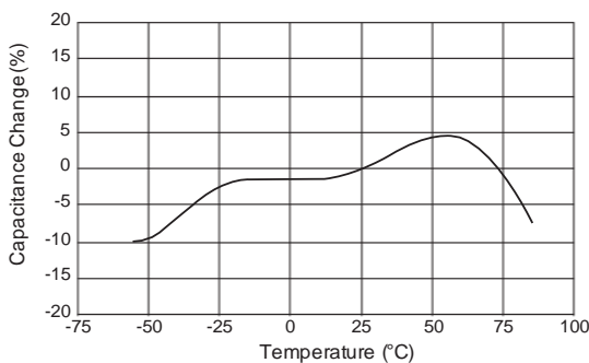
[Example of Temperature Characteristics X5R(R6)] Sample: 22µF, Rated Voltage 4VDC
