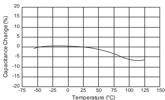
[Example of Temperature Characteristics X7R(R7)] Sample: 0.1µF, Rated Voltage 50VDC
