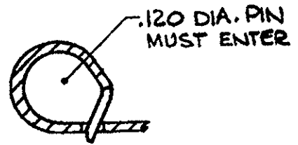
SECT. A-A
