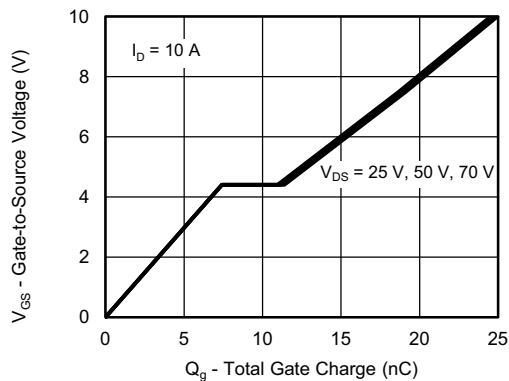
Gate Charge
