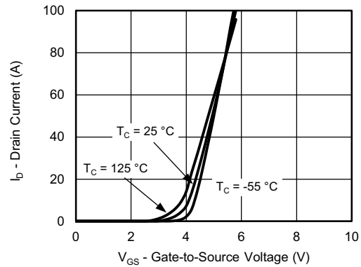
Transfer Characteristics
