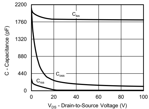
Capacitance
