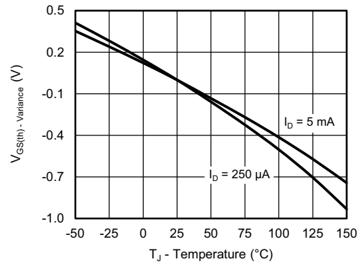
Threshold Voltage
