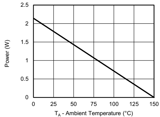
Power, Junction-to-Ambient
