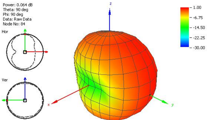
Figure 14. Radiation Pattern at 750 MHz of FXUB70 Port 1.
