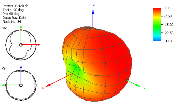
Figure 18. Radiation Pattern at 925 MHz of FXUB70 Port 1.
