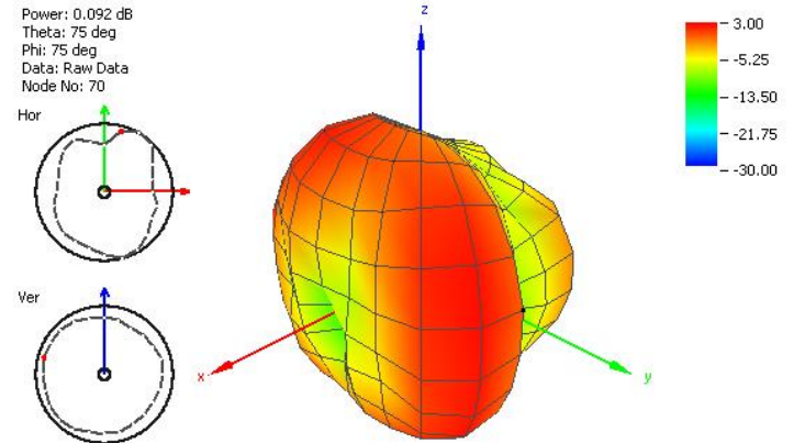
Figure 29. Radiation Pattern at 2100 MHz of FXUB70 Port 2.
