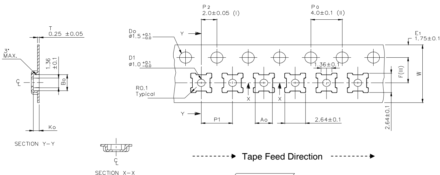
Figure 32. Tape and Reel Specifications 12-lead 2x2x0.55 mm QFN
