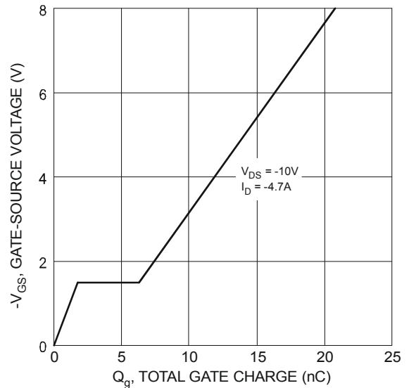
Figure 21 Gate-Charge Characteristics
