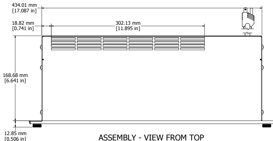
ASSEMBLY - VIEW FROM TOP
