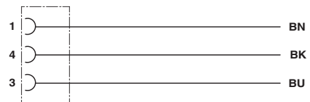
Contact assignment of the M 8 sockets, 3-pos.
