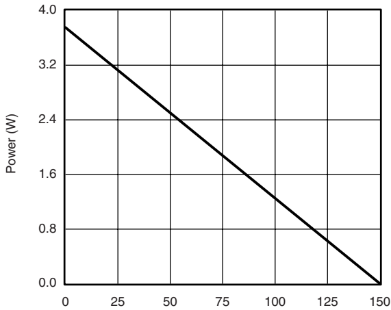
Power, Junction-to-Foot
