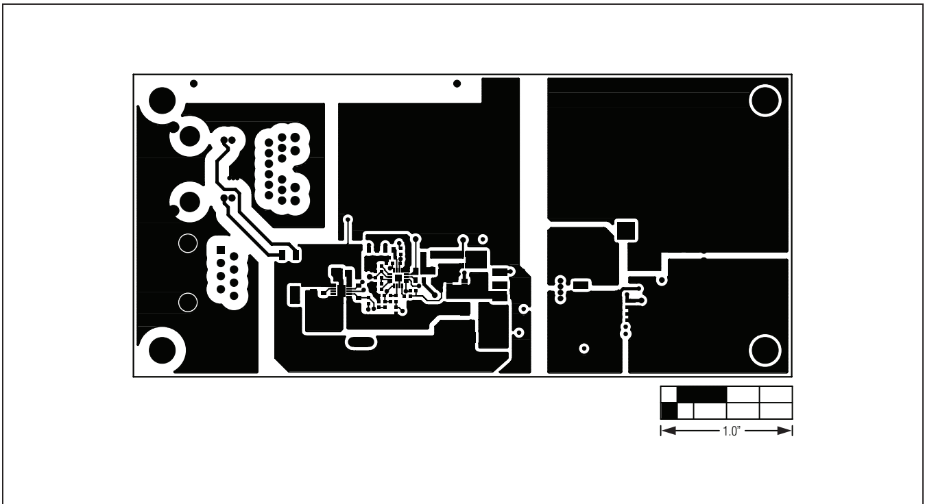
Figure 4. MAX5974C EV Kit PCB Layout—Component Side
