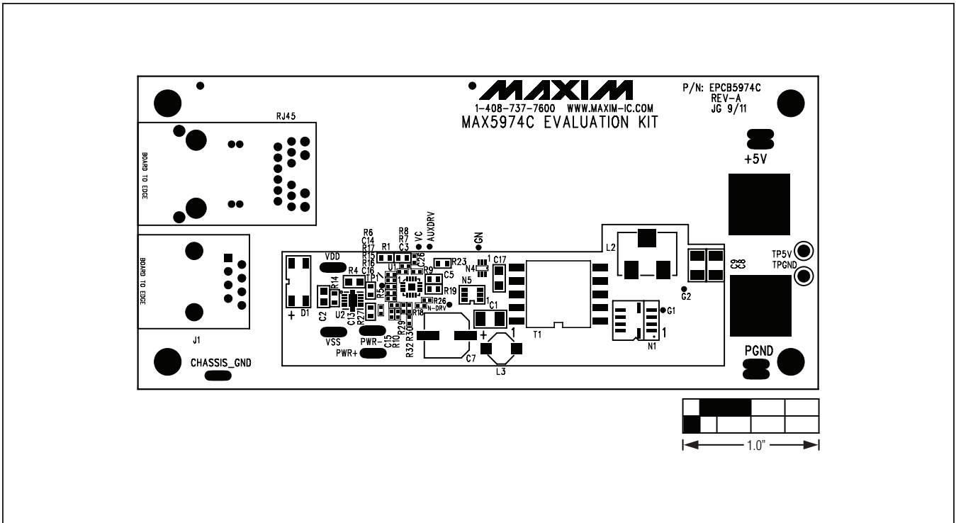
Figure 3. MAX5974C EV Kit Component Placement Guide—Component Side
