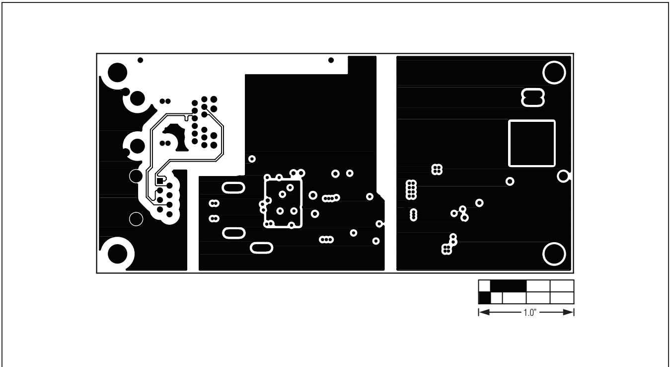
Figure 5. MAX5974C EV Kit PCB Layout—GND Layer 2
