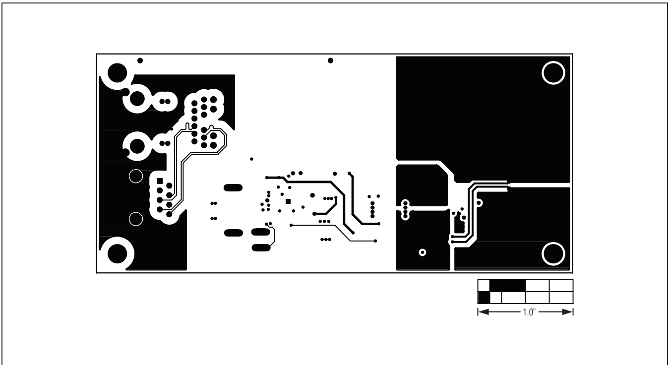
Figure 6. MAX5974C EV Kit PCB Layout—Signal Layer 3
