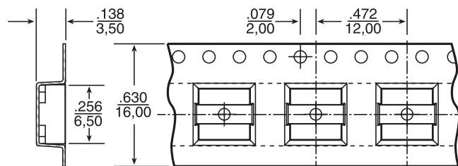
TAPE & REEL LAYOUT
