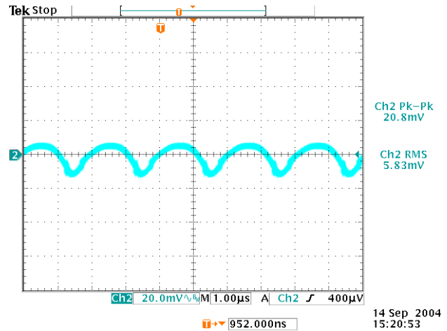
Figure 12: Output ripple & noise at 12Vin, 2.5V/4A out
