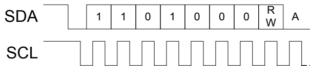
Figure 23. I 2 C Address Operation
