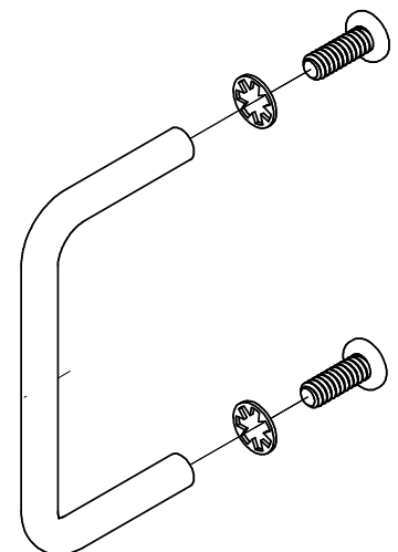
TYPICAL HANDLE ASSEMBLY
