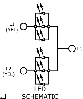
LED SCHEMATIC
