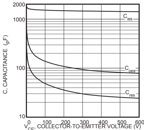
FIGURE 7, Capacitance vs Collector-To-Emitter Voltage
