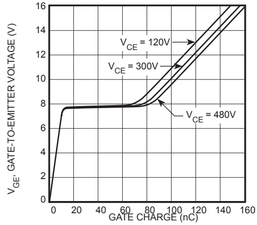
FIGURE 6, Gate Charge
