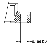
VARIATION 04 .156±.002 DIA. MOUNTING HOLE
