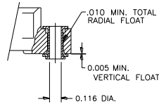
VARIATION 03 .116±.003 I.D. FLOATING EYELET
