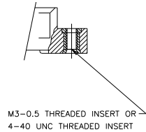
VARIATIONS 07 AND 08 THREADED INSERT
