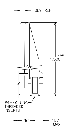
MOUNTING OPTION CODE #78
