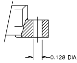
VARIATION 02 .128±.003 DIA. MOUNTING HOLE
