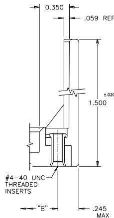
MOUNTING OPTION CODE #68
