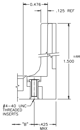
MOUNTING OPTION CODE #58
