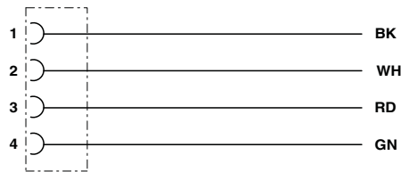
Contact assignment of 7/8" plugs/sockets, cable type 410
