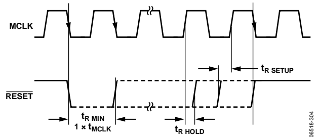
Figure 46. RESET Timing Synchronous to MCLK
