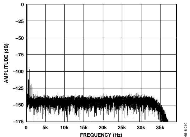
Figure 11. Low Power Mode, FFT, 1 kHz, -0.5\text{ dB} Input Tone, 256x Decimation Rate
