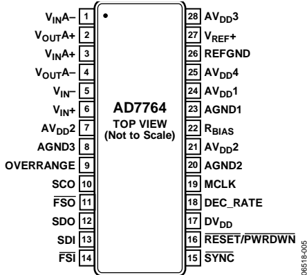
Figure 5. Pin Configuration
