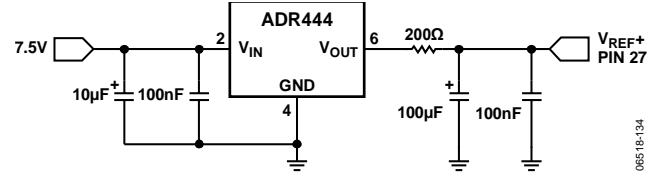
Figure 54. Reference Connection
