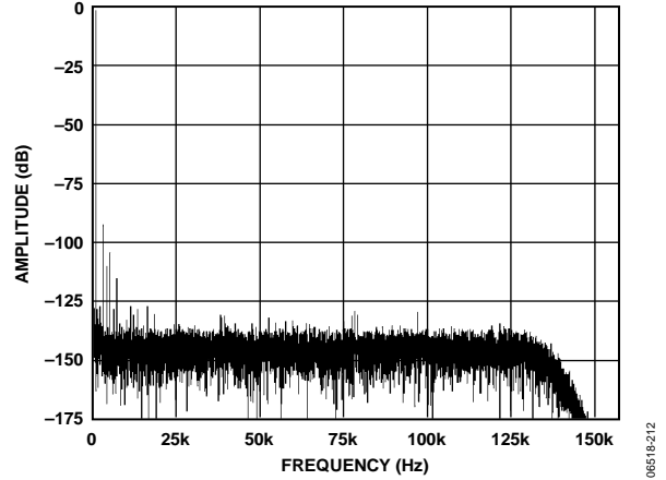
Figure 9. Low Power Mode, FFT, 1 kHz, -0.5\text{ dB} Input Tone, 64x Decimation Rate
