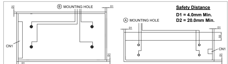
Fig. 3: Mounting Hole Locations and the Safety Distance
