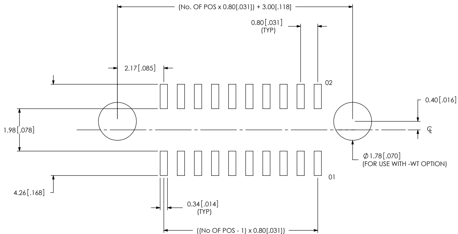
FIG 5 (SEMX-110-02-03.0-XX-D-WT SHOWN)
