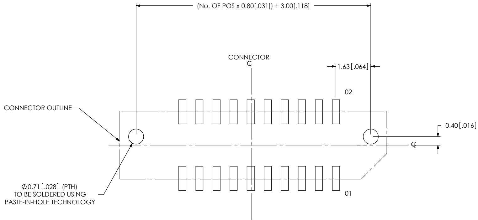
FIG 3 (SEM-X-110-02-03.0-XX-D-WT SHOWN) (SAME AS FIG 1, DIFFERENT AS SHOWN)
