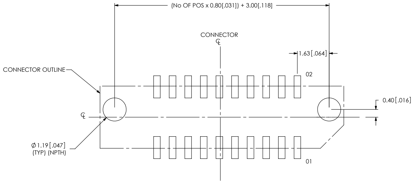
FIG 2 (SEM-110-02-03,0-XX-D-LC SHOWN) (SAME AS FIG 1, DIFFERENT AS SHOWN)
