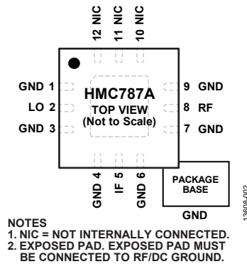
Figure 2. Pin Configuration
