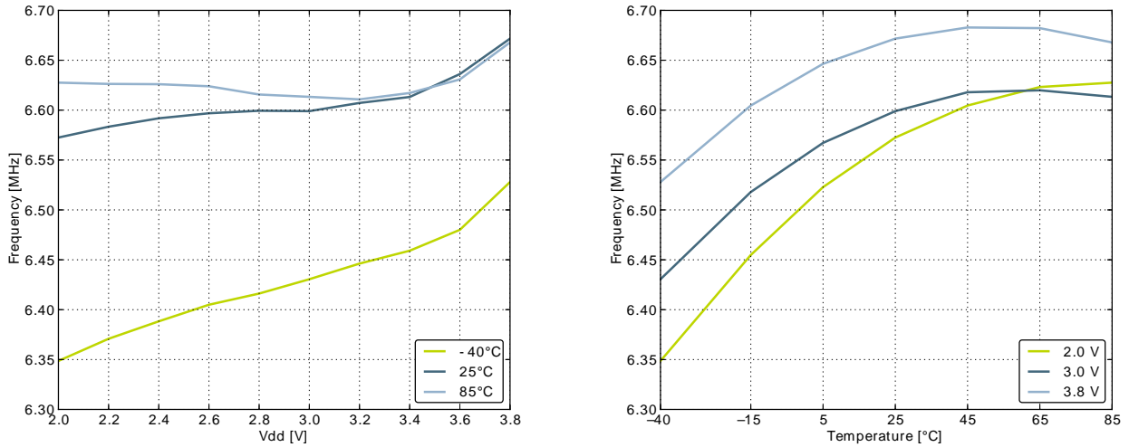
Figure 3.23. Calibrated HFRCO 11 MHz Band Frequency vs Supply Voltage and Temperature
