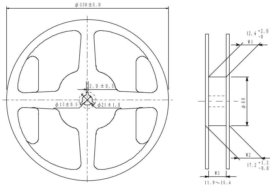
Figure 1 Reel dimension(Unit:mm)
