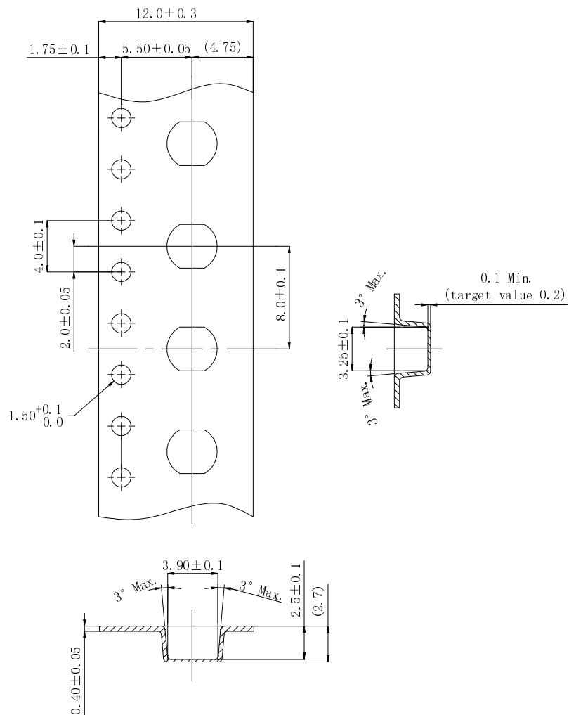
Figure 2 Tape dimension (Unit:mm)
