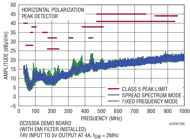
Figure 3. LT8640S Demo Circuit DC2530A EMI Performance (14V input from VEMI, with EMI filter, I_{OUT} = 4A )
