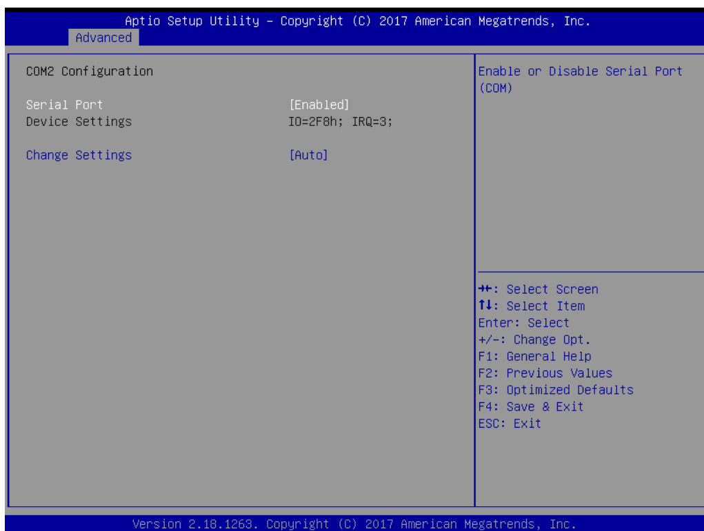
Figure 3.12 COM2 Configuration
