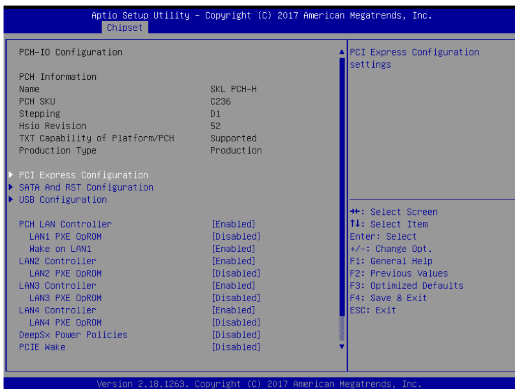
Figure 3.23 PCH-IO Configuration
