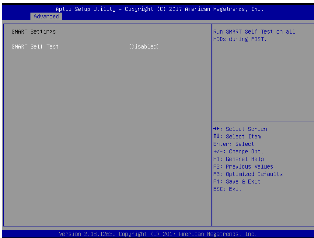
Figure 3.9 SMART Setting
