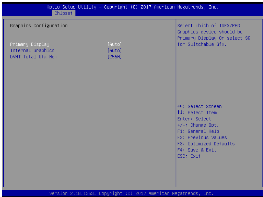
Figure 3.20 Graphics Configuration
