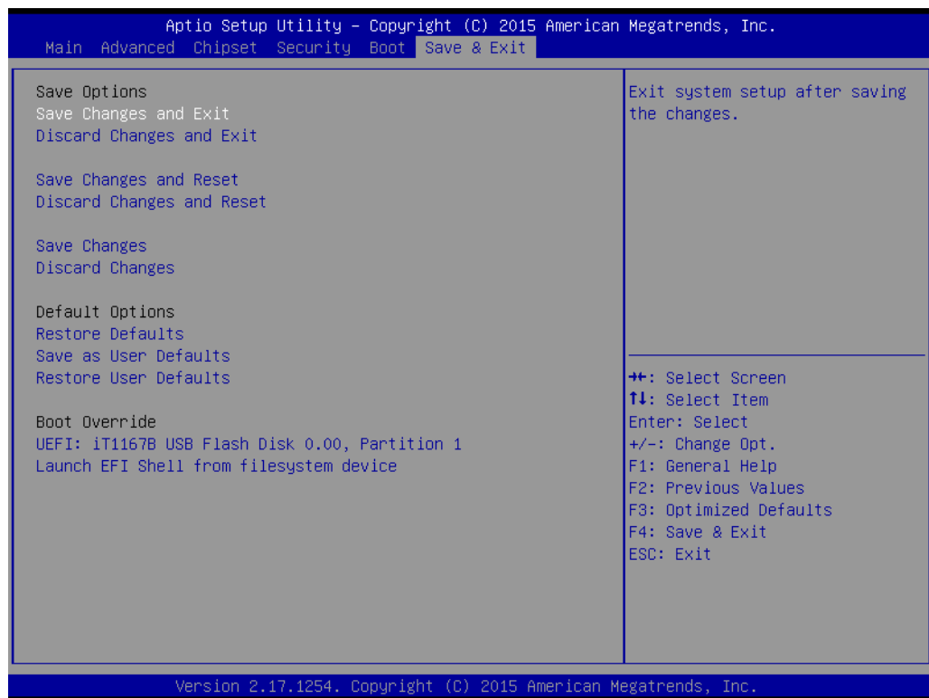
Figure 3.30 Save & Exit
