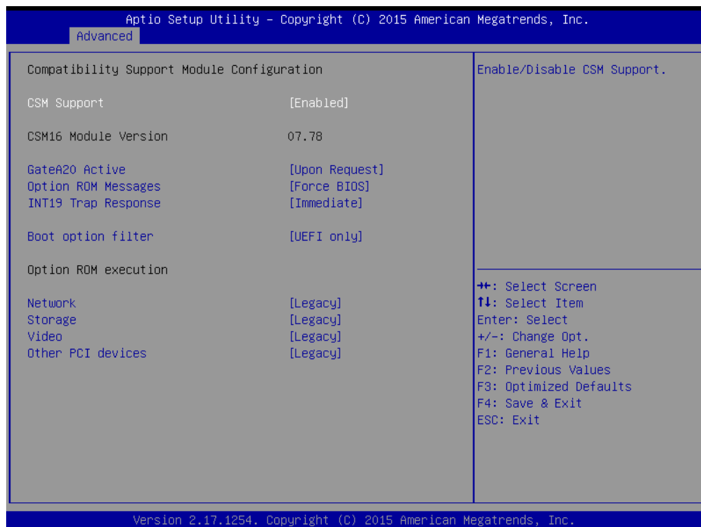
Figure 3.17 CSM16 Parameters
