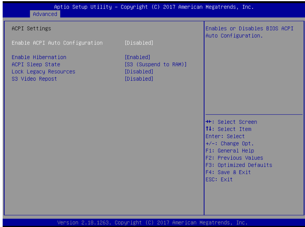
Figure 3.8 ACPI Settings
