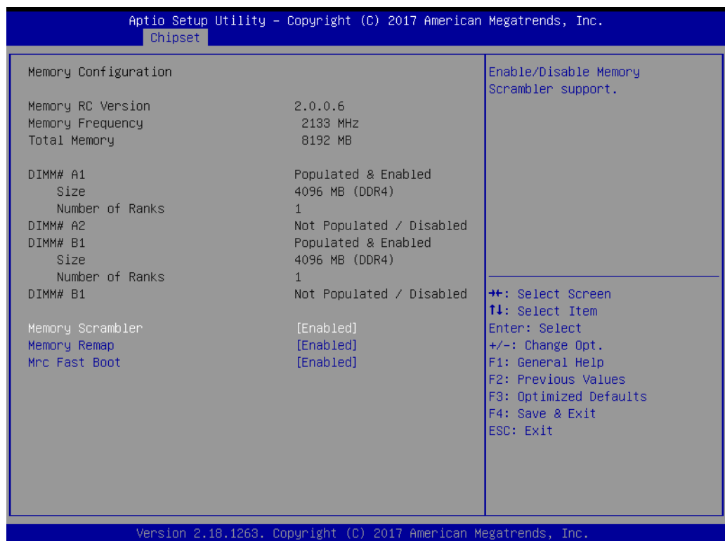
Figure 3.22 Memory Configuration
