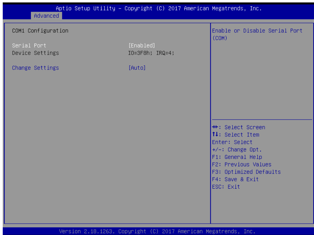
Figure 3.11 COM1 Configuration
