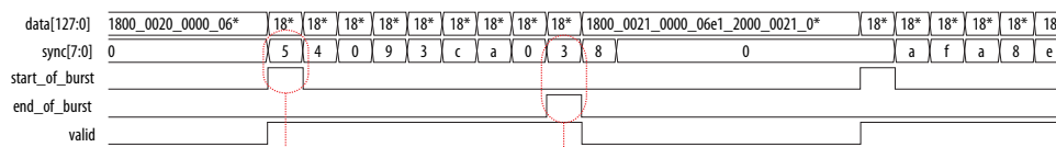
Figure 9. Source Waveform for Burst Mode (Sync)
