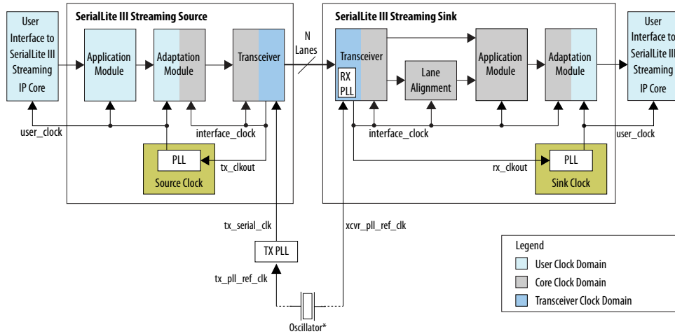
Figure 14. Standard Clocking Mode Structure for Intel Arria 10 Devices
