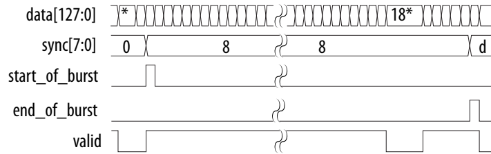
Figure 12. Sink Waveform for Continuous Mode
