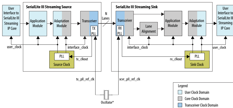
Figure 15. Standard Clocking Mode Structure for Stratix V or Arria V Devices
