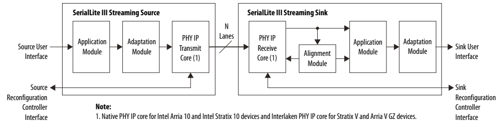
Figure 6. SerialLite III Streaming IP Core Duplex Core
