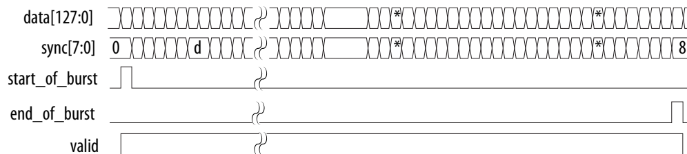
Figure 10. Source Waveform for Continuous Mode
