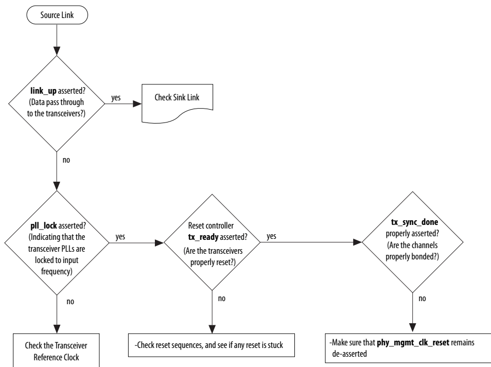
Figure 23. Source Core Link Debugging Flow Chart
