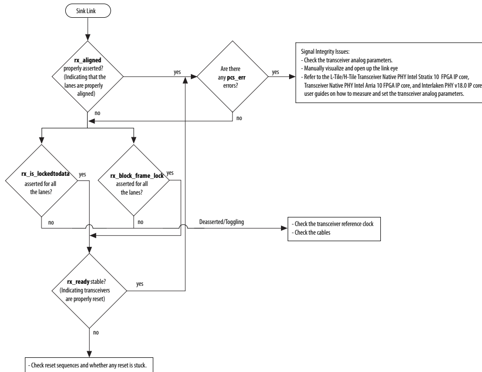
Figure 24. Sink Core Link Debugging Flow Chart
