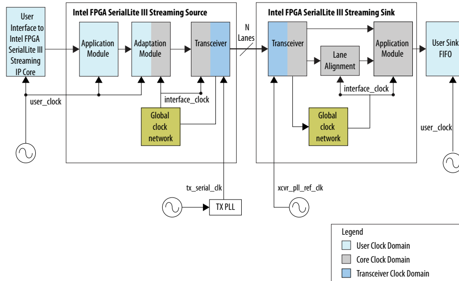
Figure 22. Same Source and Sink User Frequencies, with Different Crystal Oscillators for Intel Arria 10, Stratix V and Arria V GZ Devices
