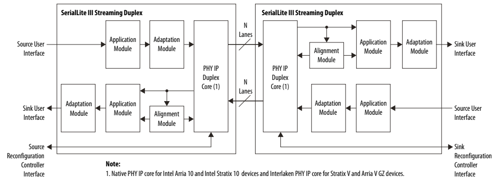
Figure 6. SerialLite III Streaming IP Core Duplex Core
