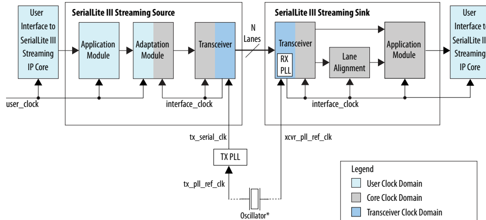
Figure 17. Advanced Clocking Mode Structure for Intel Arria 10 Devices
