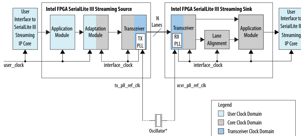
Figure 18. Advanced Clocking Mode Structure for Stratix V or Arria V Devices
