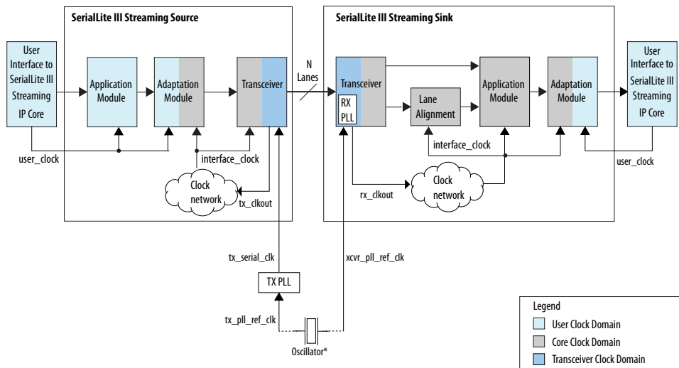
Figure 13. Standard Clocking Mode Structure in Intel Stratix 10 Devices
