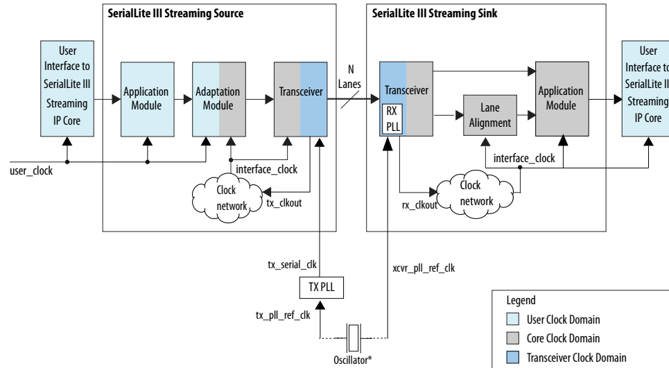
Figure 16. Advanced Clocking Mode Structure for Intel Stratix 10 Devices
