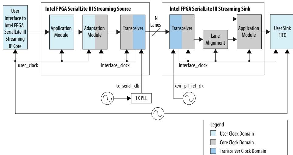
Figure 20. Same Source and Sink User Clock Frequencies from Same Crystal Oscillator for Intel Arria 10, Stratix V and Arria V GZ Devices
