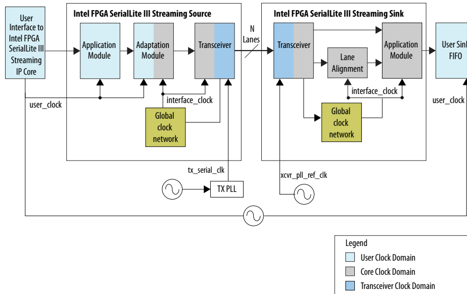
Figure 20. Same Source and Sink User Clock Frequencies from Same Crystal Oscillator for Intel Arria 10, Stratix V and Arria V GZ Devices
