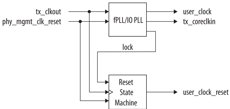
Figure 7. Clock Generator Block Diagram
