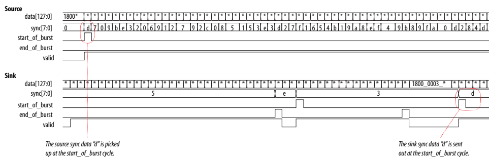
Figure 11. Sink Waveform for Burst Mode
