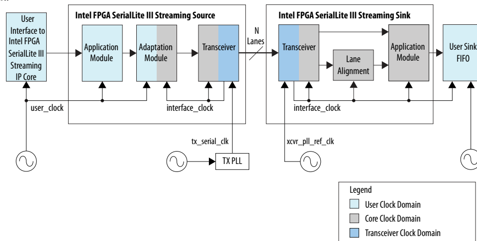
Figure 22. Same Source and Sink User Frequencies, with Different Crystal Oscillators for Intel Arria 10, Stratix V and Arria V GZ Devices
